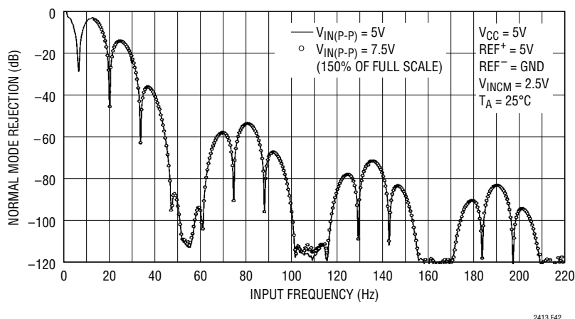
Figure 42. Measured Input Normal Mode Rejection vs Input Frequency with Input Perturbation of 150% of Full Scale
